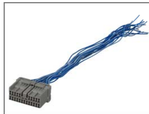
QJ273 23 pin connector
