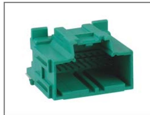
QJ289-2 20 pin horizontal type connector (Green)
